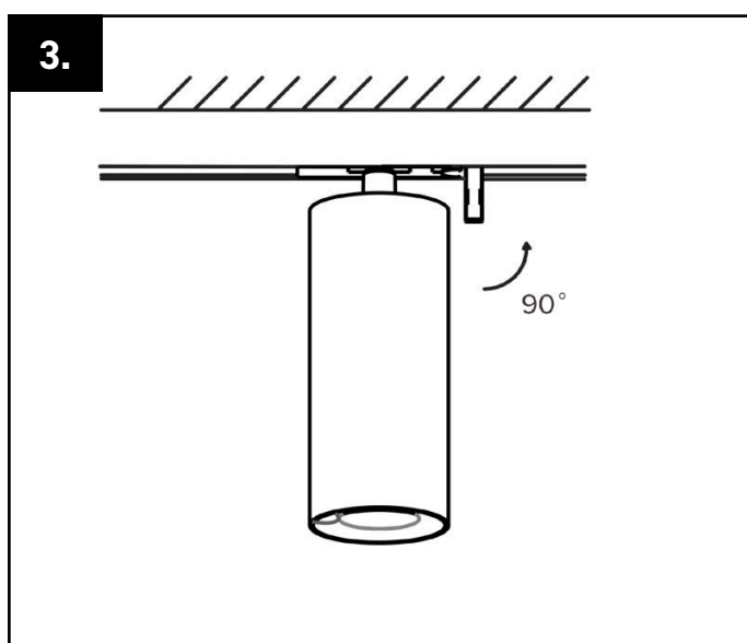
Click the fixing lever into the track adapter
