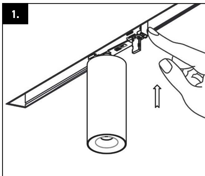
Insert the Altera spot light into the track
