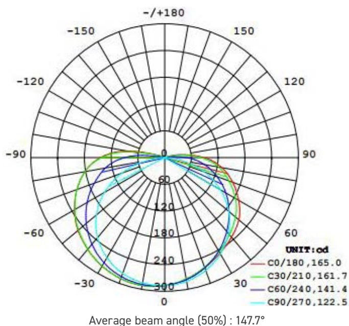
B Plane Distribution Diagram
