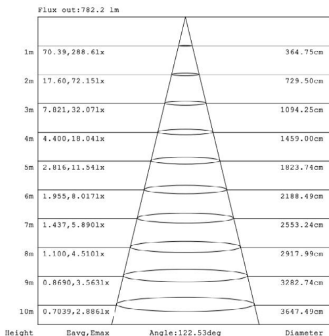
Illuminance Distance Curve
