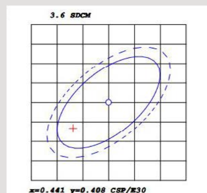
CIE1931 Chromaticity Diagram
