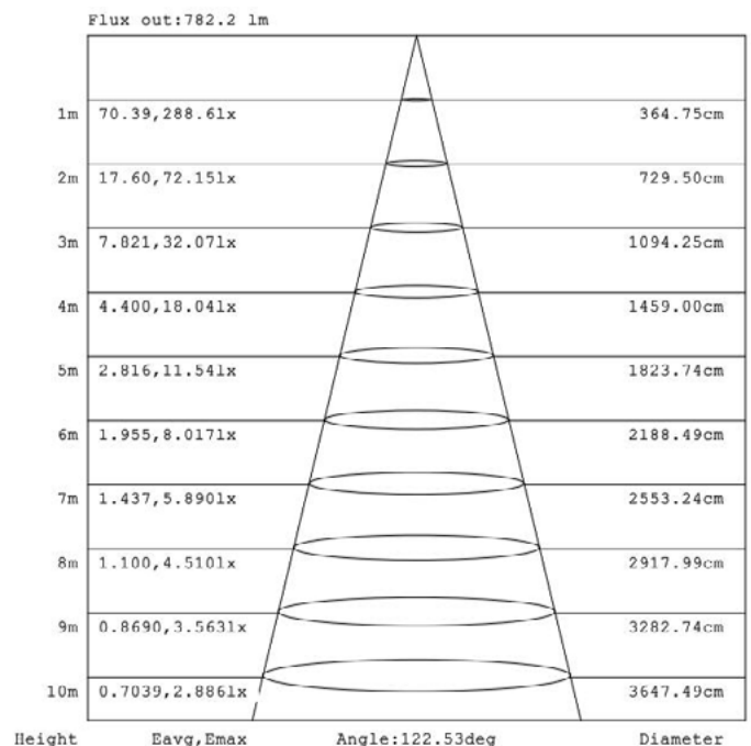
Illuminance Distance Curve
