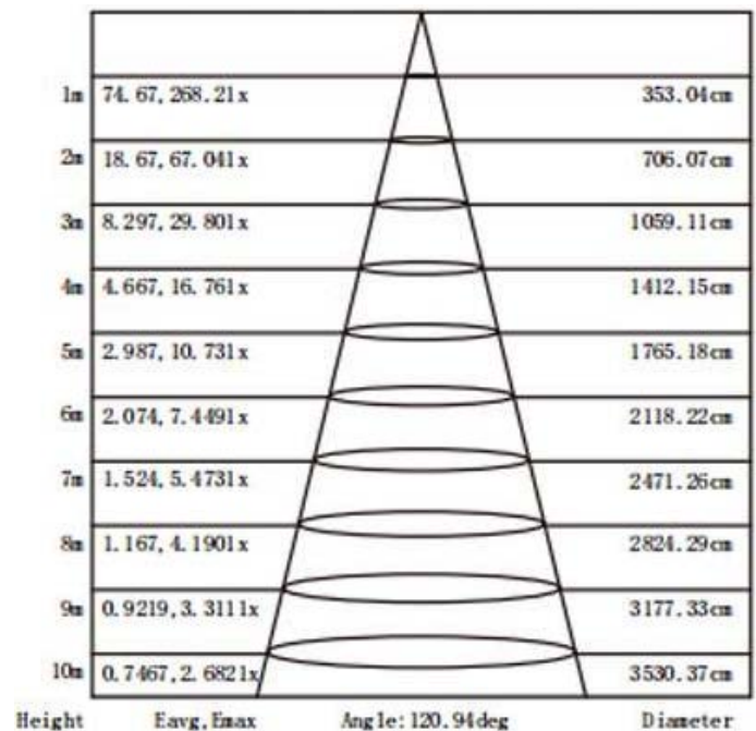
Illuminance Distance Curve
