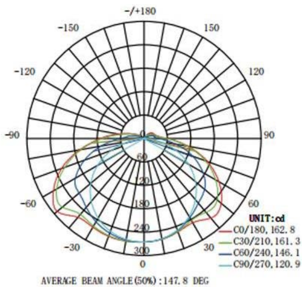
B Plane Distribution Diagram
