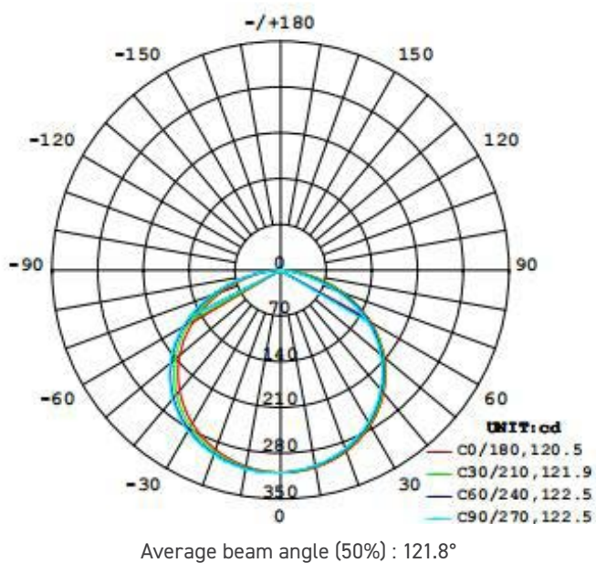
B Plane Distribution Diagram
