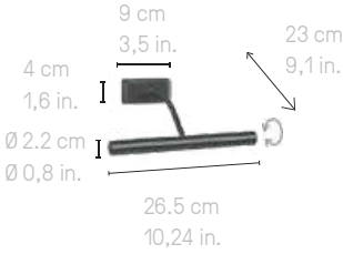
picture light 9004 BR
