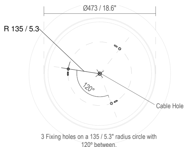
Fixing Dimensions
