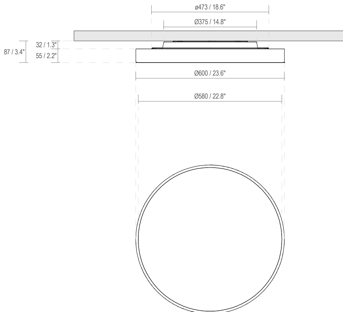
Fixing Dimensions
