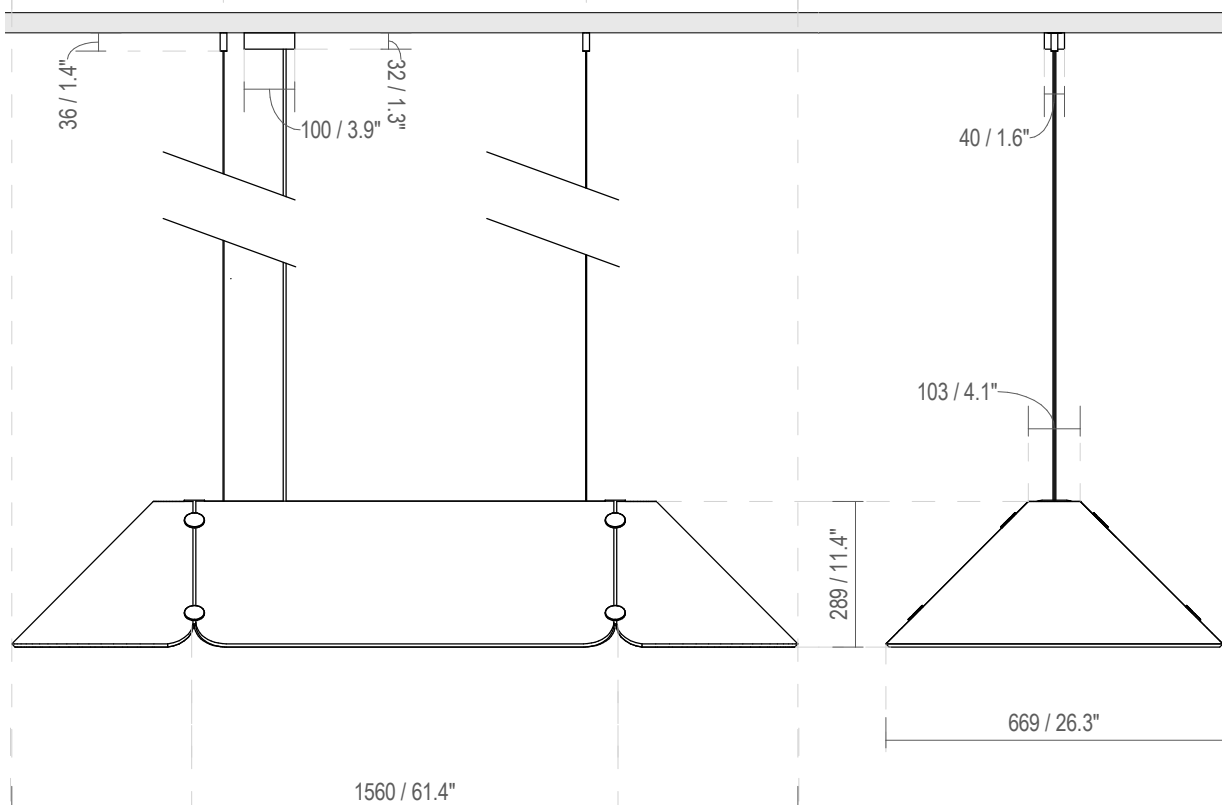
Fixing Dimensions
