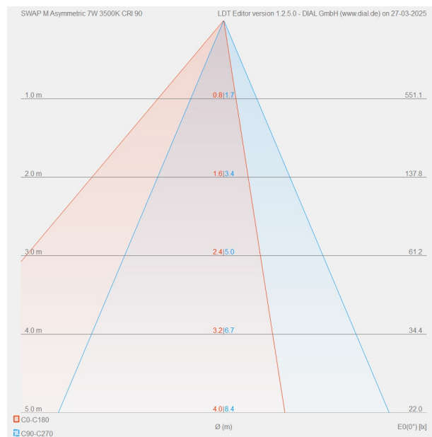
CONICAL DIAGRAM
