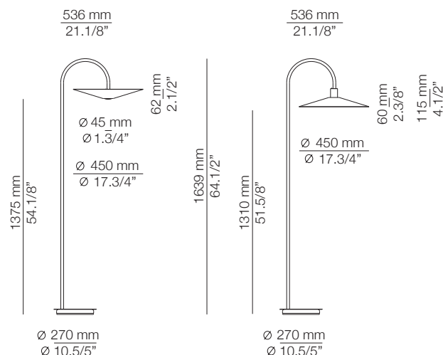
BEL_4149L: with large metall shade Ø 450mm
