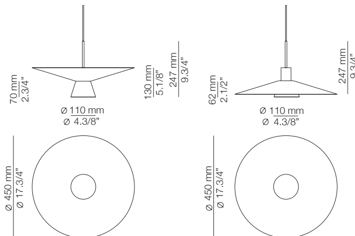
BEL_4145 with large metal shade Ø 450mm + glass shade
