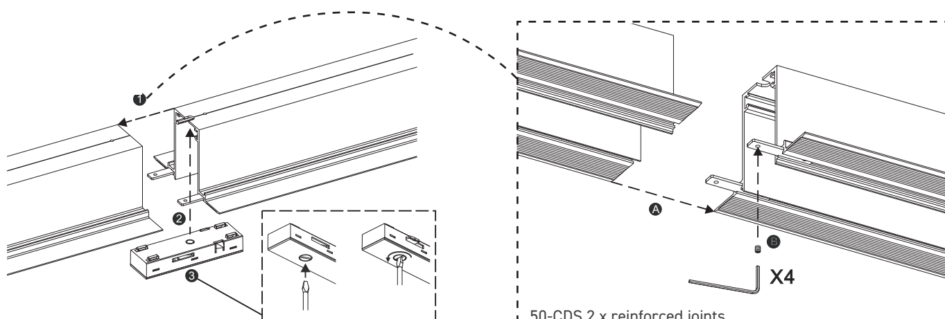
50-CDS 2 x reinforced joints
