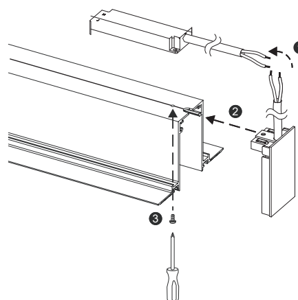
30-CDS End cap 2m power cable
