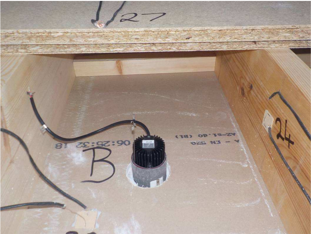
Photo 2.1.6 – Downlight B
