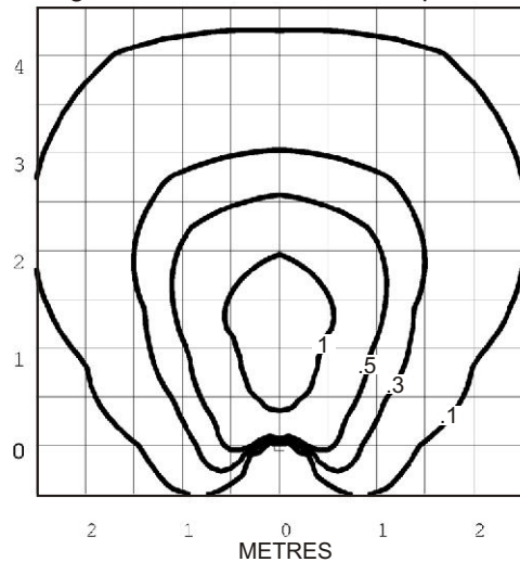
Isolux Lumens Plot - Footcandles = Isolux figures divided by 10.76
