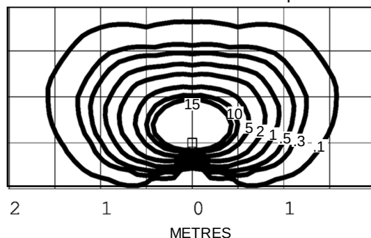
Mouse Lite 20 watt G4 Bi-Pin lamp - Lens height 400mm (15¾")
