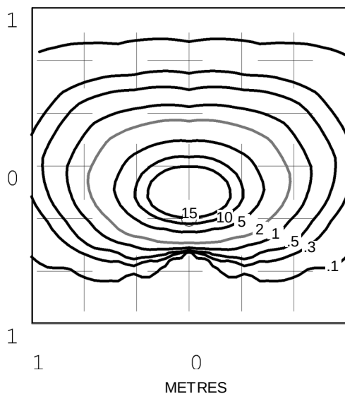
Mouse Lite 20 watt G4 Bi-Pin lamp - Lens height 400mm (15¾")
