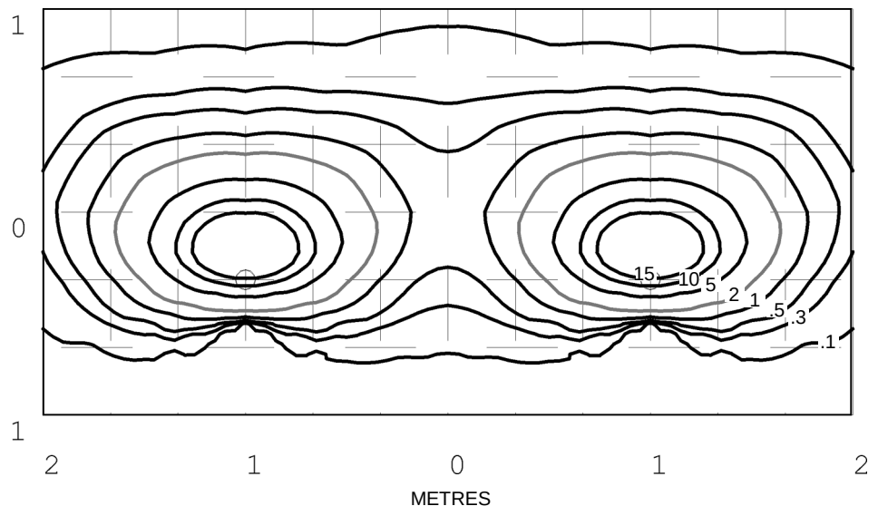
Mouse Lite 20 watt G4 Bi-Pin lamp - Lens height 400mm (15¾")
