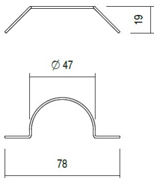
ML053 Spring for Aura Round S
