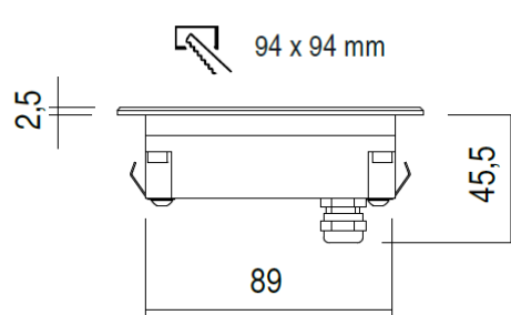
AURA ROUND L
