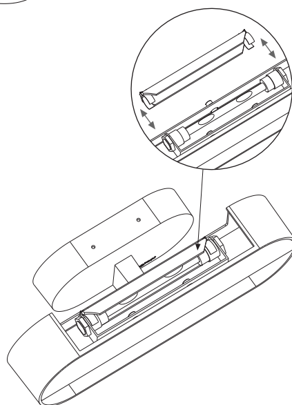
R7s 120W ECO 114mm
